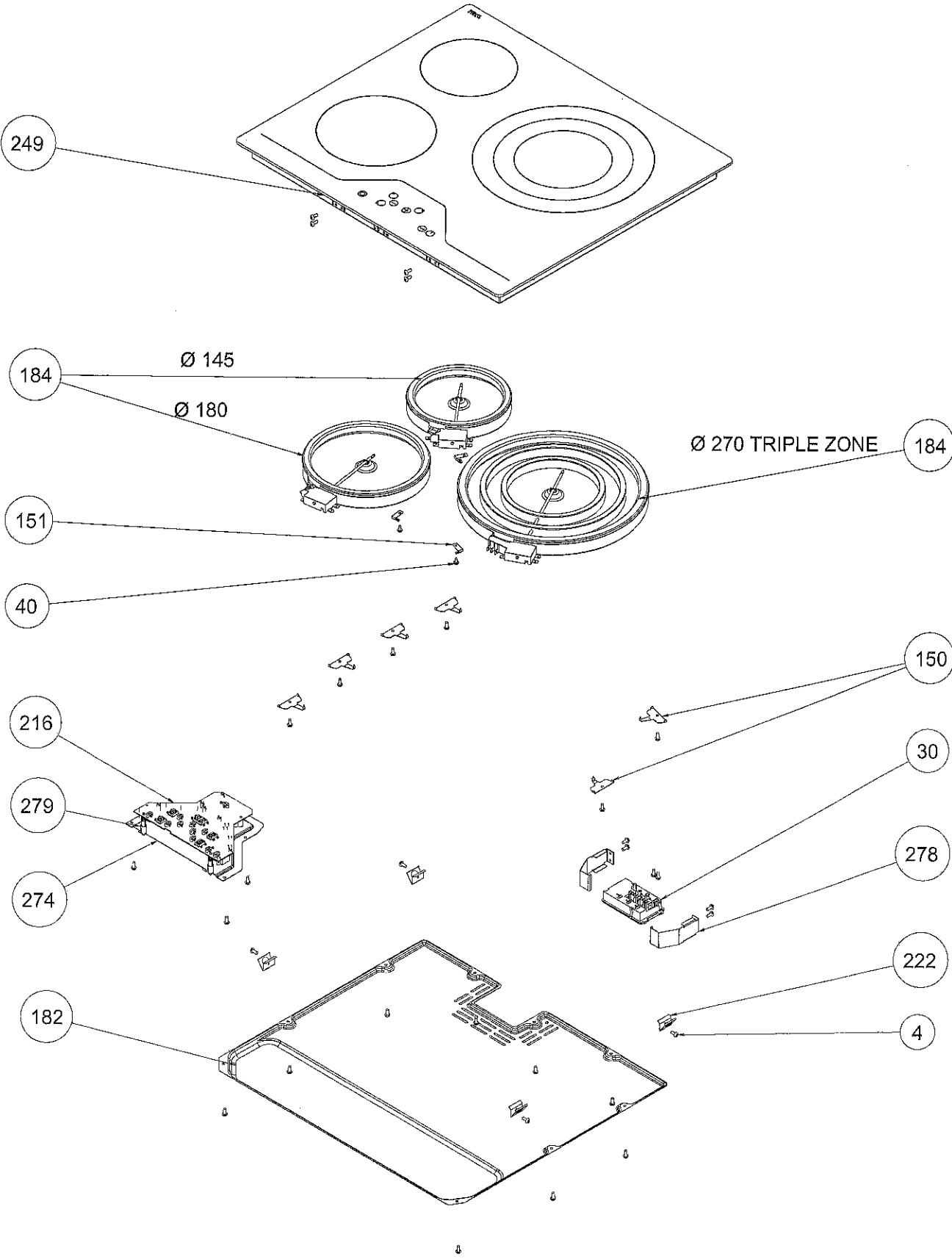
EXPLODED VIEW - FRONT SIDE TOUCH CONTROL VITROCERAMIC HOB ASSEMBLY
